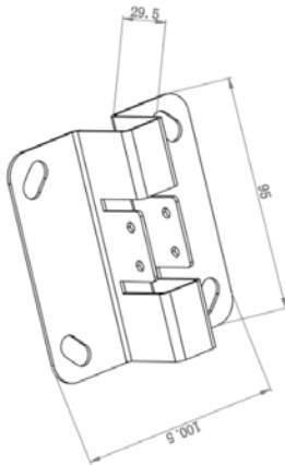
Mounting plate dimensions
