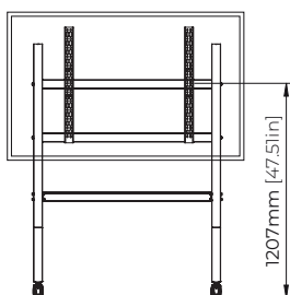
Min. Screen Height Assembly
