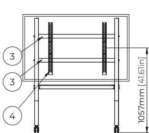
Min. Screen Height Assembly
