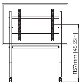
Middle Screen Height Assembly
