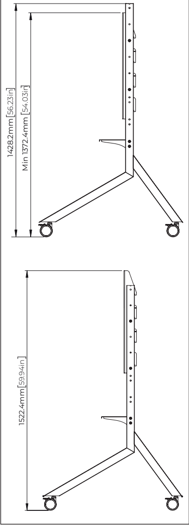
Side View Lowest Horizontal Bar Assembly
