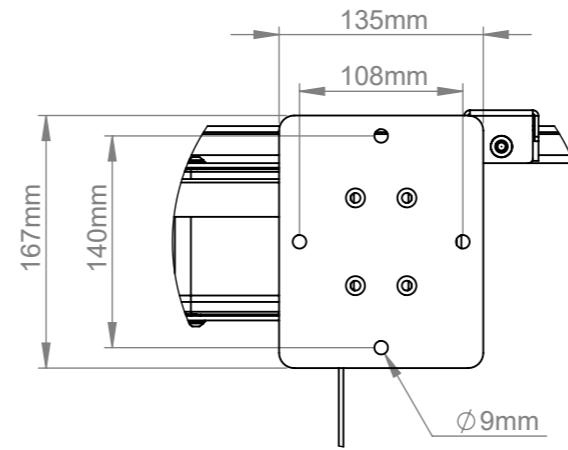
FLOOR PLATE SCALE 1 : 5
