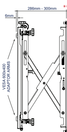
SIDE VIEW EXTENDED
