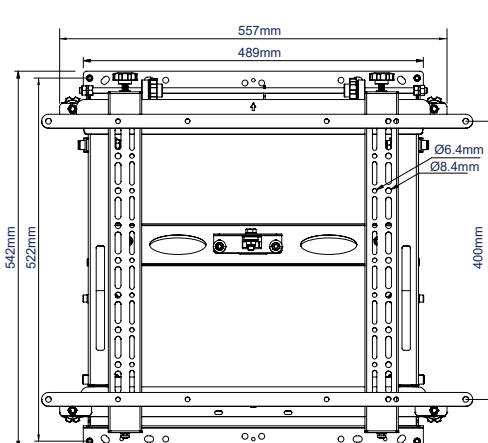
FRONT VIEW WITH ADAPTOR ARMS
