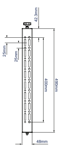
INTERFACE ARM
