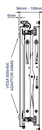
SIDE VIEW CLOSED
