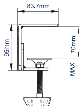
DESK CLAMP
