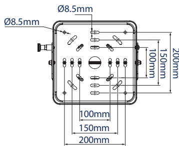
BOTTOM VIEW / INTERFACE PLATE
