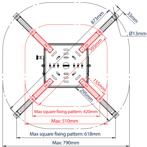
INTERFACE WITH LONG EXTENSION LEGS & SHORT EXTENSION LEGS
